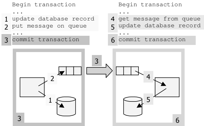
Fig. 15. Transactional messaging
