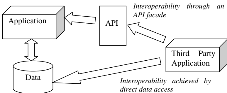
Fig. 8. Integration options
