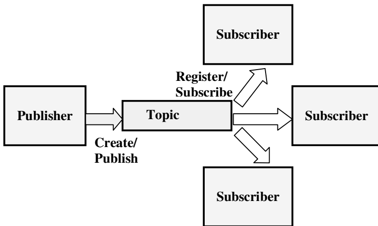
Fig. 18. Publish-Subscribe messaging
