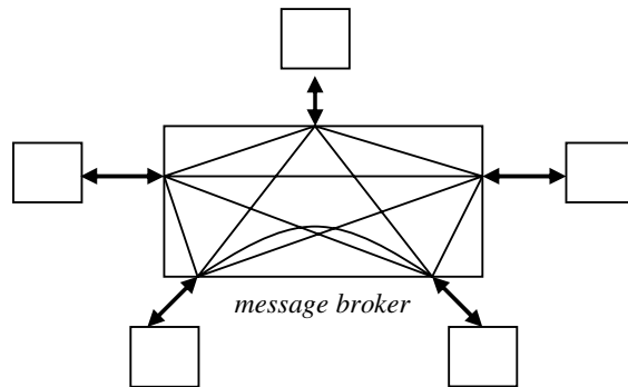
Fig. 34. Eliminating a point-to-point architecture with a message broker.
